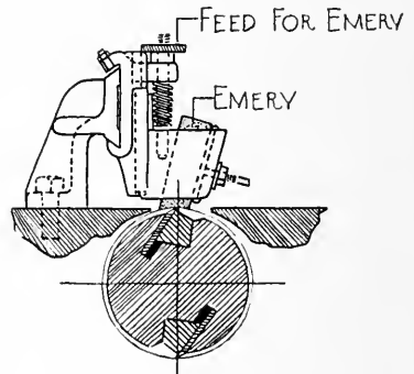
FIG. 142. JOINTER FOR HAND PLANERS.
